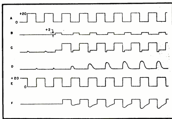
Fig. 5. Waveforms at various points in the circuit of Fig. 4. Clock A is shown as a square wave although a half-wave rectified sine wave can be used.
