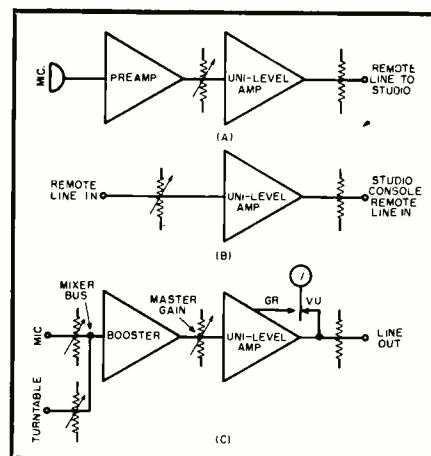
Fig. 5. (A) Typical application of Type BA-9-A at remotes. (B) Application at studio for unattended remotes. (C) How amplifier may be used in most consoles.
