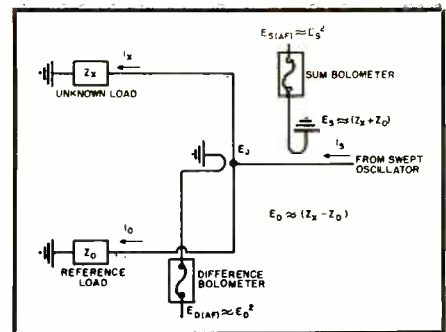
Fig. 1. Schematic diagram showing basic operating principles of reflectometer.
