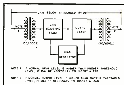
Fig. 6. Block diagram of “uni-level” amplifier. Note that pads may be necessary to adjust input and output levels.
