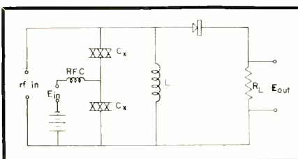
Fig. 1. "Resonant" dielectric amplifier circuit provides gain greater than unity.
