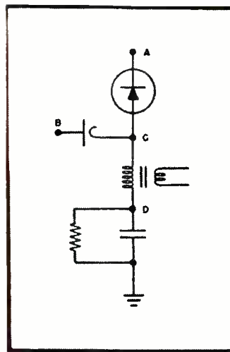
Fig. 3. The addition of a capacitor and a resistor aids in transformer primary recovery between pulses.
