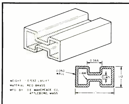
Fig. 3. Double ridge wave guide design.
