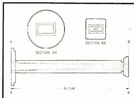
Fig. 5. Ridge to rectangular transition.
