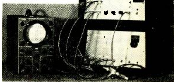
Fig. 2. Complete indicator set up for operation. The reflectometer is in front; oscilloscope at left; scanning oscillators at top and bottom, right; ratio-measuring unit, right, center.
