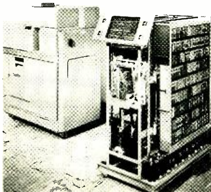
Experimental all-transistor computing unit is shown uncovered at the right with high-speed punching unit at left.
